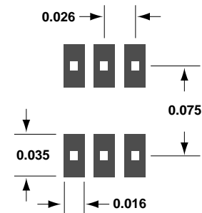
Figure 22. PCB Pad Layout (dimensions in inches).
