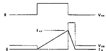
図2 動作波形 Operating waveforms
