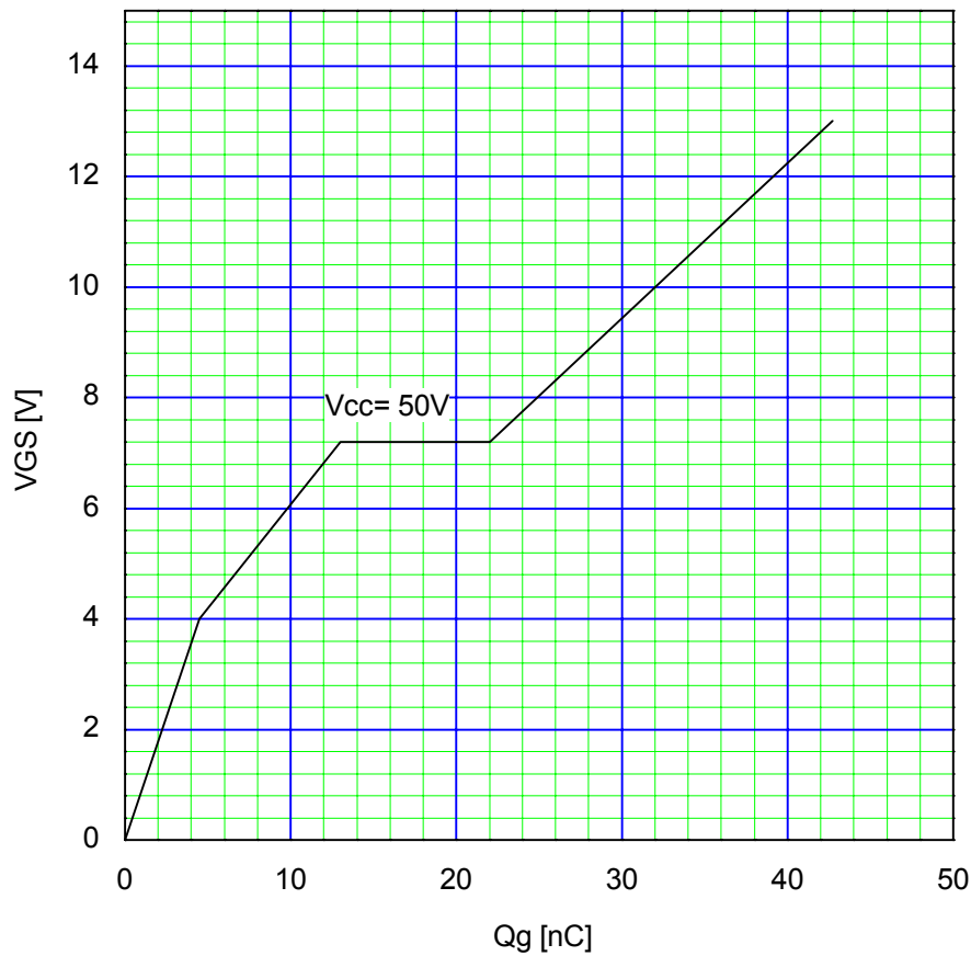
Typical Gate Charge Characteristics V_{GS} = f(Q_g) : I_D = 30\text{A}, T_{ch} = 25\text{ °C}
