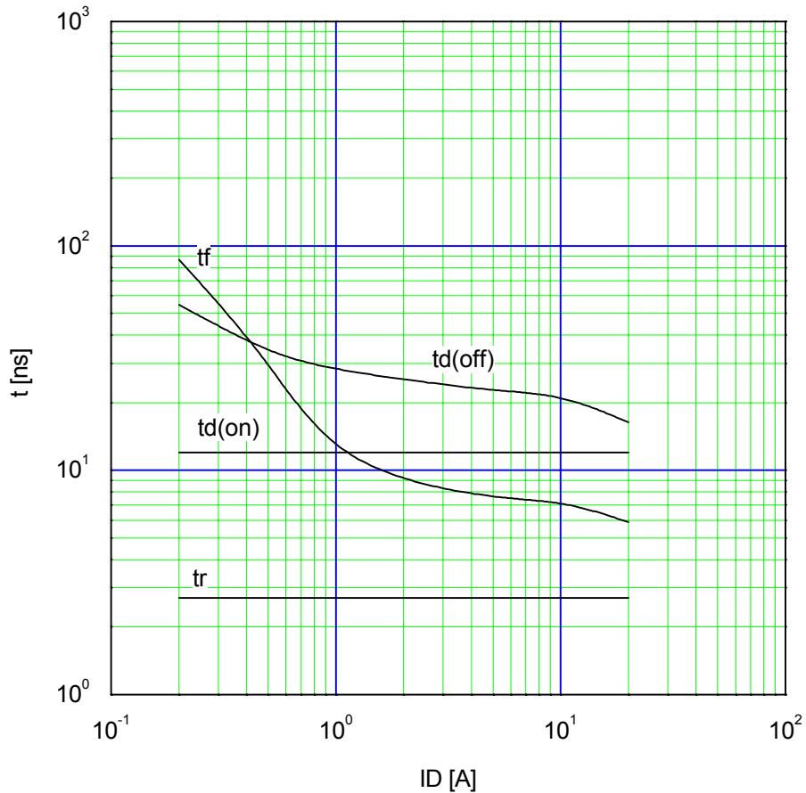
Typical Switching Characteristics vs. I_D t=f(I_D):V_{cc}=48\text{V},V_{GS}=10\text{V},R_G=10\ \Omega
