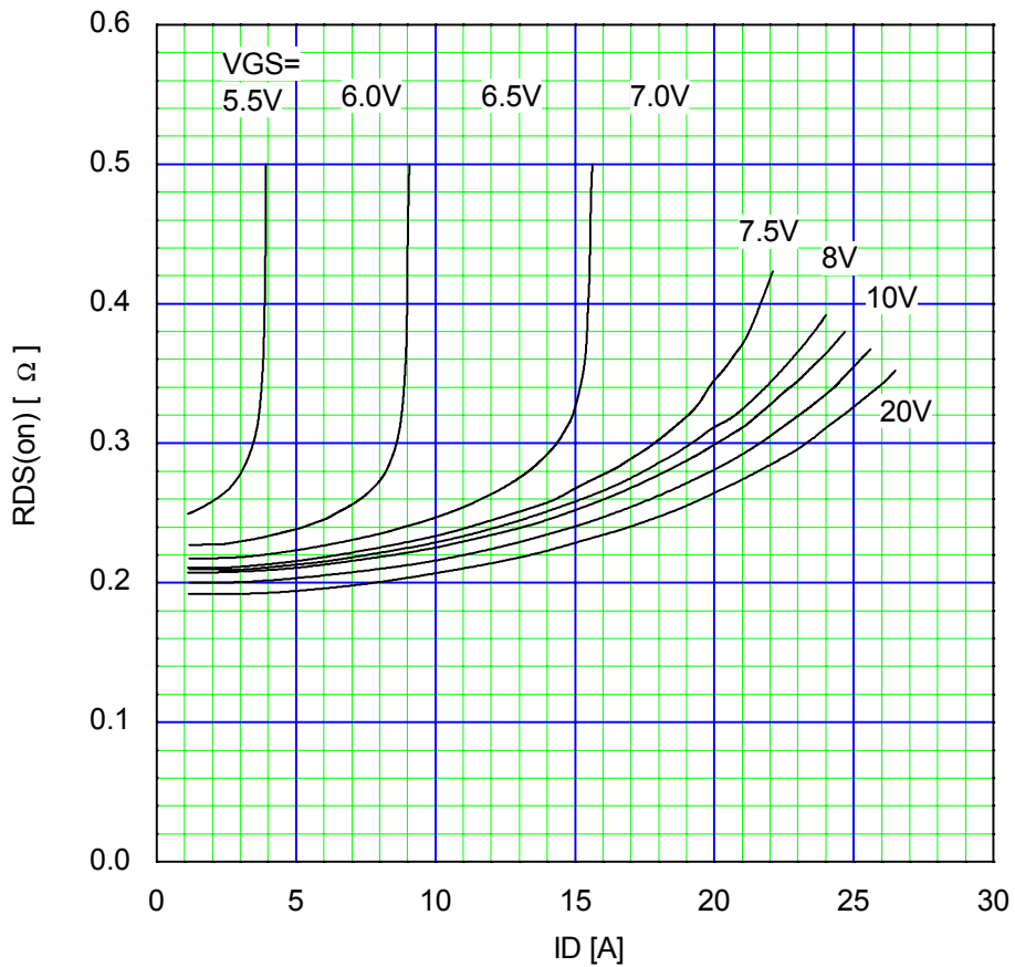
Typical Drain-Source on-state Resistance R_{DS(on)}=f(I_D):80\ \mu\text{s}\ \text{pulse}\ \text{test}, T_{ch}=25^\circ\text{C}
