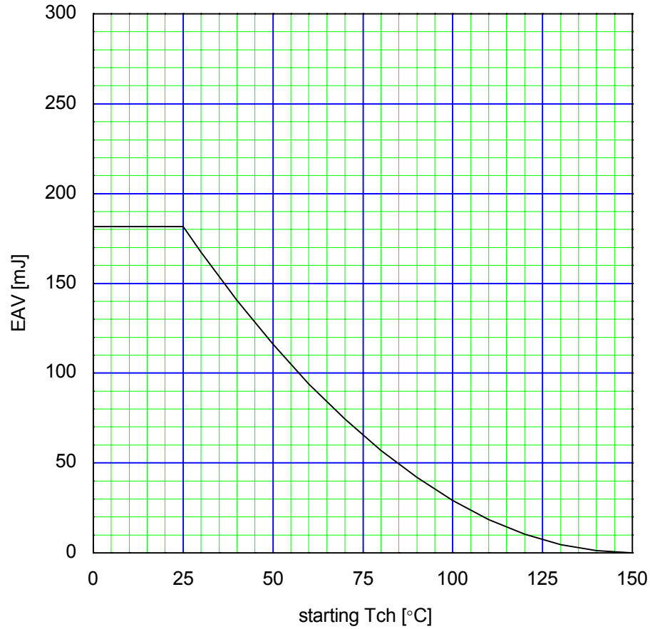
Maximum Avalanche Energy vs. starting Tch E(AV)=f(\text{starting Tch}):V_{CC}=48V, I(AV)\leq 10A
