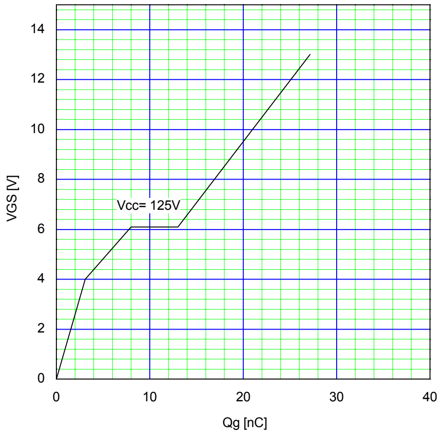
Typical Gate Charge Characteristics V_{GS}=f(Q_g):I_D=10A,T_{ch}=25^{\circ}C
