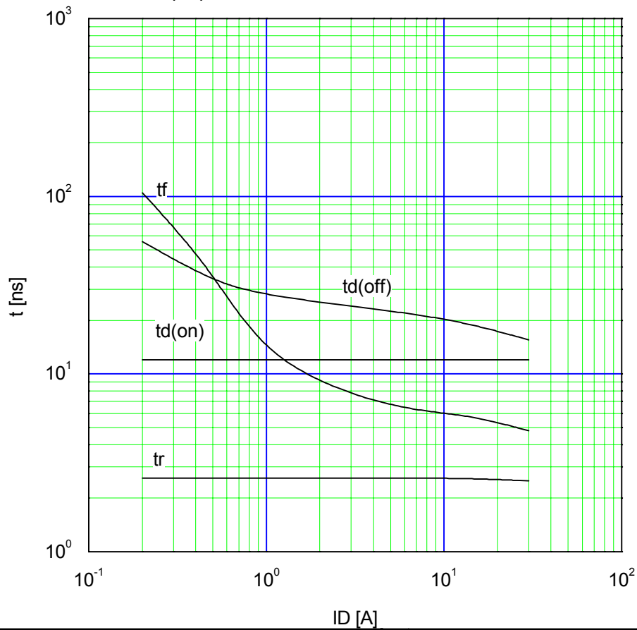
Typical Switching Characteristics vs. I_D t=f(I_D): V_{cc}=48\text{V}, V_{GS}=10\text{V}, R_G=10 \Omega
