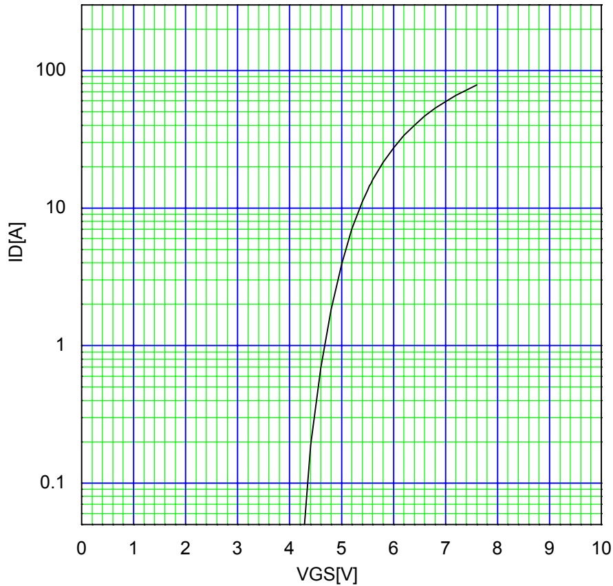
Typical Transfer Characteristic I_D=f(V_{GS}):80\mu s pulse test, V_{DS}=25V , T_{ch}=2^{\circ}C
