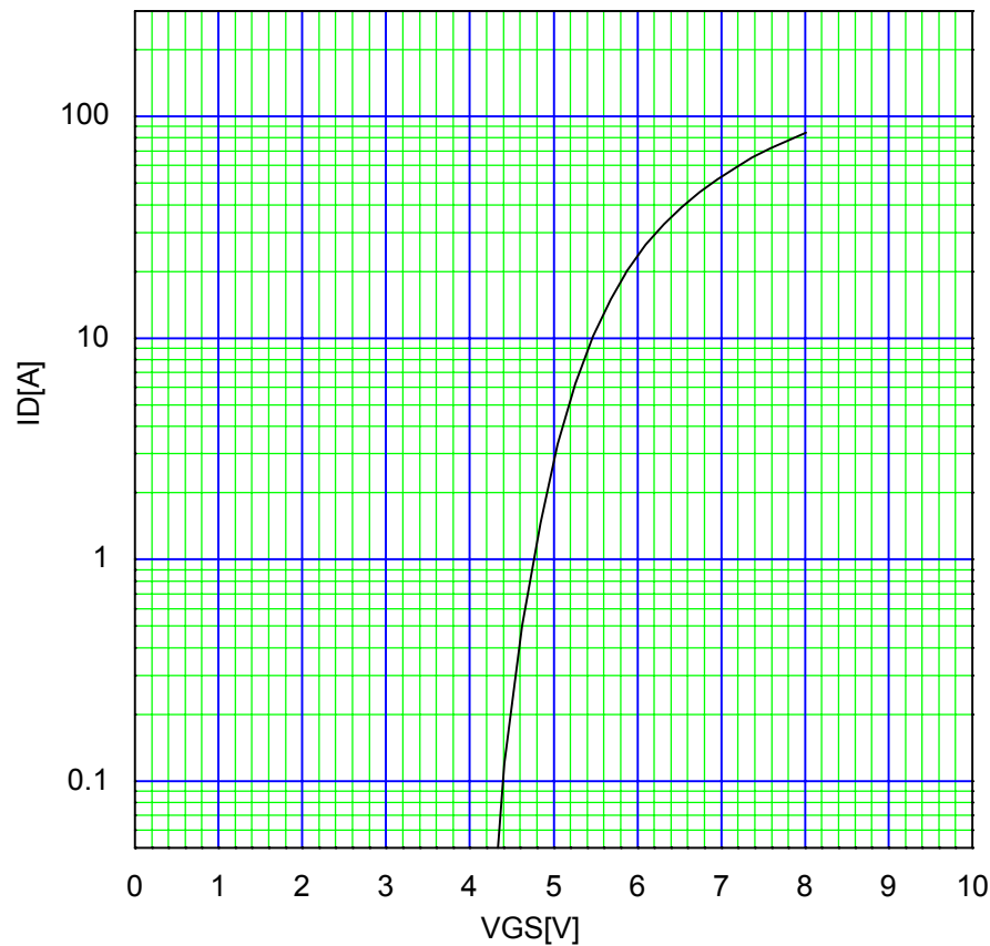
Typical Transfer Characteristic I_D = f(V_{GS}) : 80 \mu s pulse test, V_{DS} = 25\text{V} , T_{ch} = 2^\circ\text{C}
