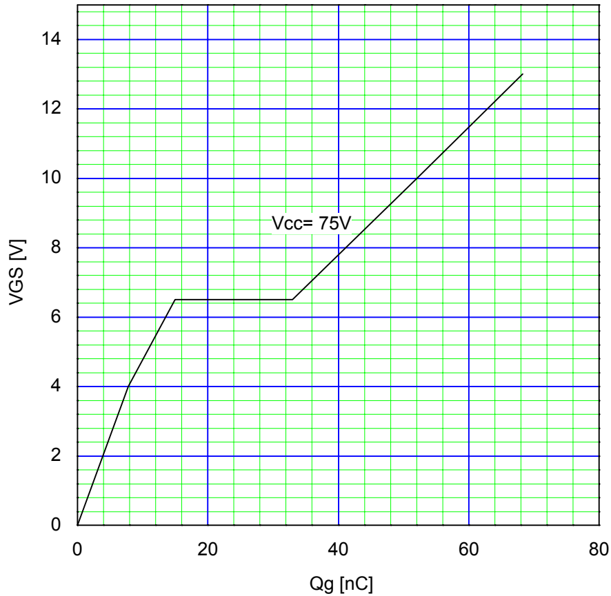
Typical Gate Charge Characteristics V_{GS}=f(Q_g):I_D=40A, T_{ch}=25^{\circ}C
