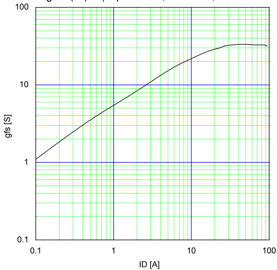
Typical Transconductance g_{fs}=f(I_D):80\mu\text{s pulse test},V_{DS}=25\text{V},T_{ch}=25^\circ\text{C}
