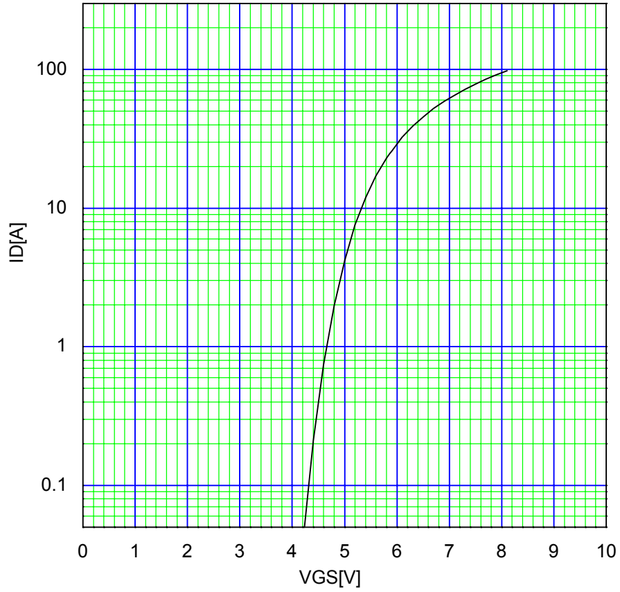
Typical Transfer Characteristic I_D=f(V_{GS}):80\mu\text{s pulse test},V_{DS}=25\text{V},T_{ch}=2^\circ\text{C}
