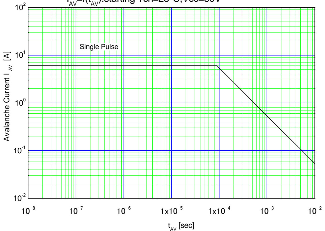
Maximum Avalanche Current Pulsewidth
