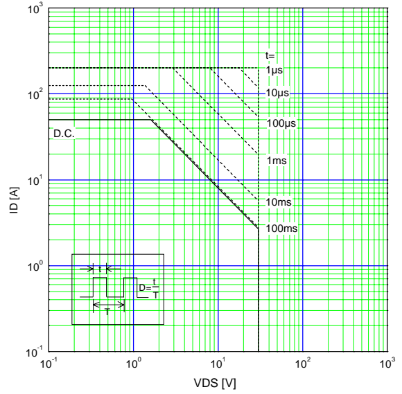
Safe operating area ID=f(V_{DS}): D=0.01, T_c=25^\circ C
