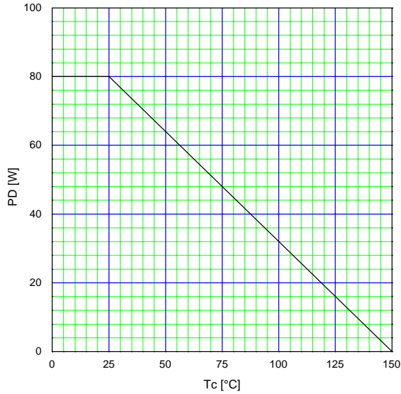
Power Dissipation PD=f(T_c)
