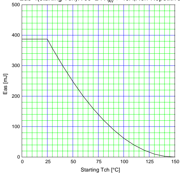
Maximum Avalanche energy vs. starting Tch E_{as}=f(\text{starting Tch}): V_{cc}=24V, I_{AV} \le 40A, \text{Non-Repitative}
