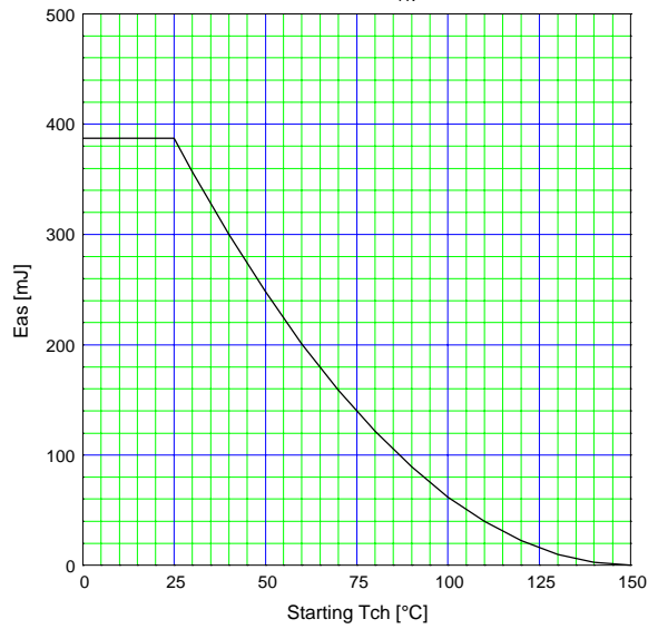
Maximum Avalanche energy vs. starting Tch E_{as}=f(\text{starting Tch}): V_{cc}=24V_A, I_A \le 40A, \text{Non-Repetitive}
