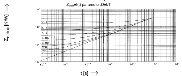
Transient Thermal Impedance
