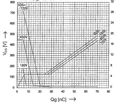
Typical Gate Charge Characteristic V_{GS} = f(Q_g) ; I_D = 5\text{A}
