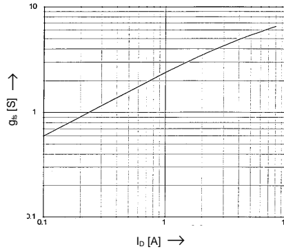
Typical Transconductance g_m = f(I_D) ; 80μs pulse test; V_{DS} = 25\text{V} ; T_C = 25^\circ\text{C}
