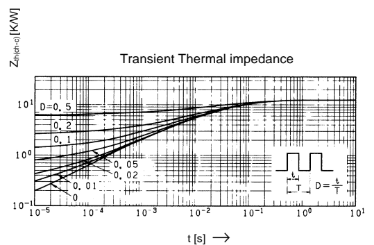
Z_{th(j-c)}
