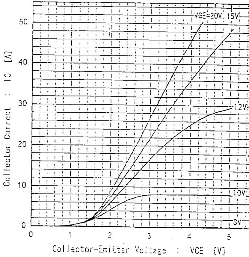
Collector Current vs. Collector-Emitter Voltage Tj=125°C
