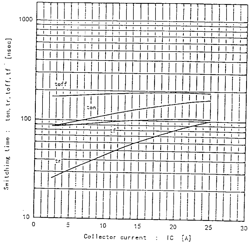
Switching time vs. Collector current V_{CC}=300V, R_G=16\Omega, V_{GE}=\pm 15V, T_j=25^\circ C
