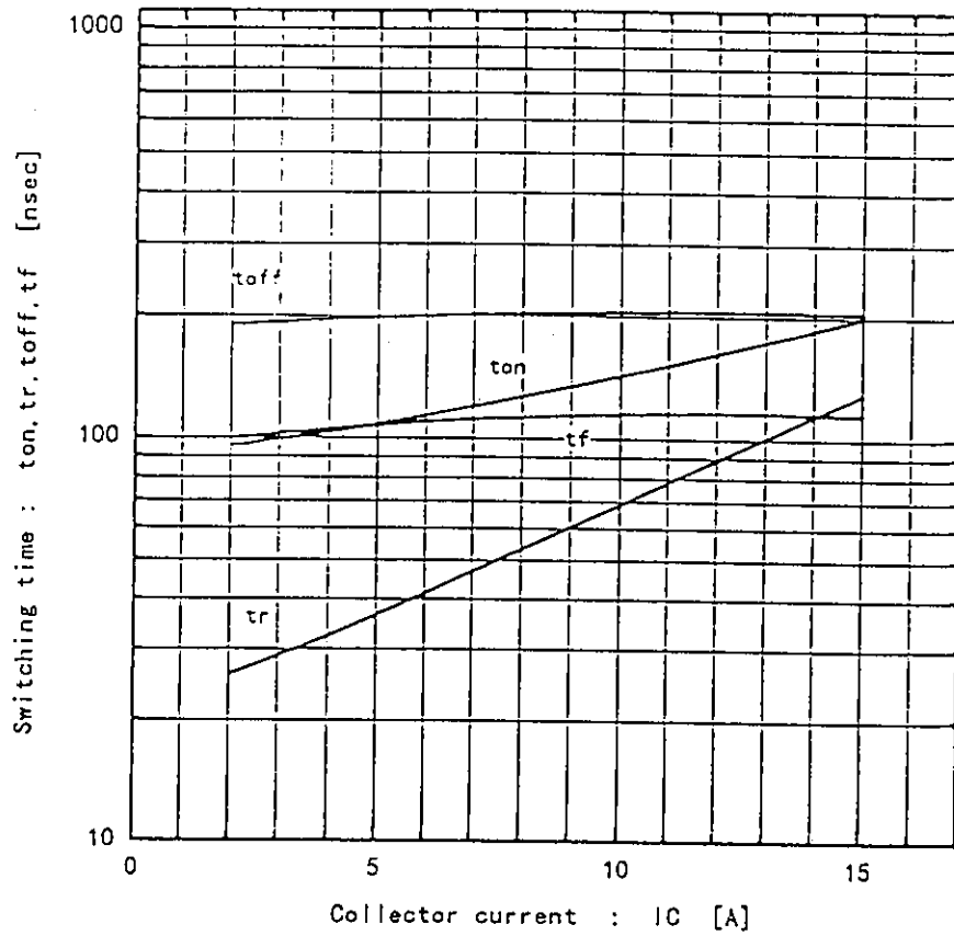
Switching time vs. Collector current V_{cc}=300V, R_G=22\Omega, V_{GE}=\pm 15V, T_j=125^\circ C
