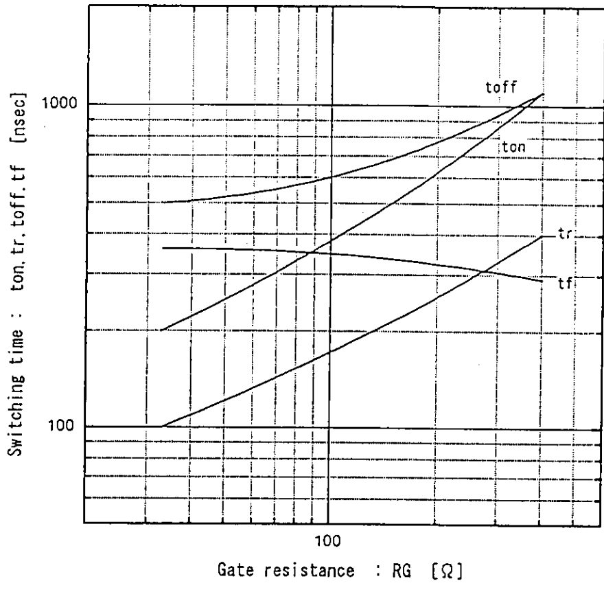
Switching time vs. R_G V_{CC}=600V, I_C=5A, V_{GE}=\pm 15V, T_j=125^\circ C
