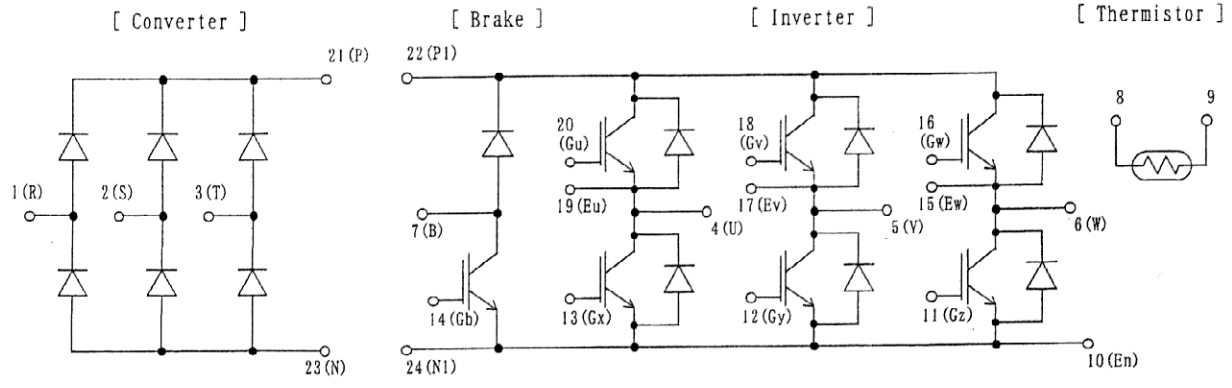
2. Equivalent circuit
