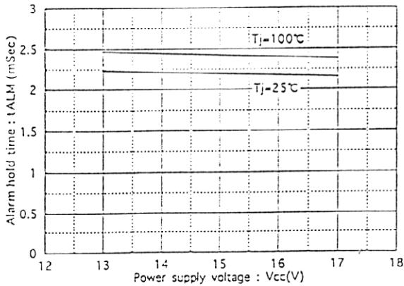
Alarm hold time vs. Power supply voltage
